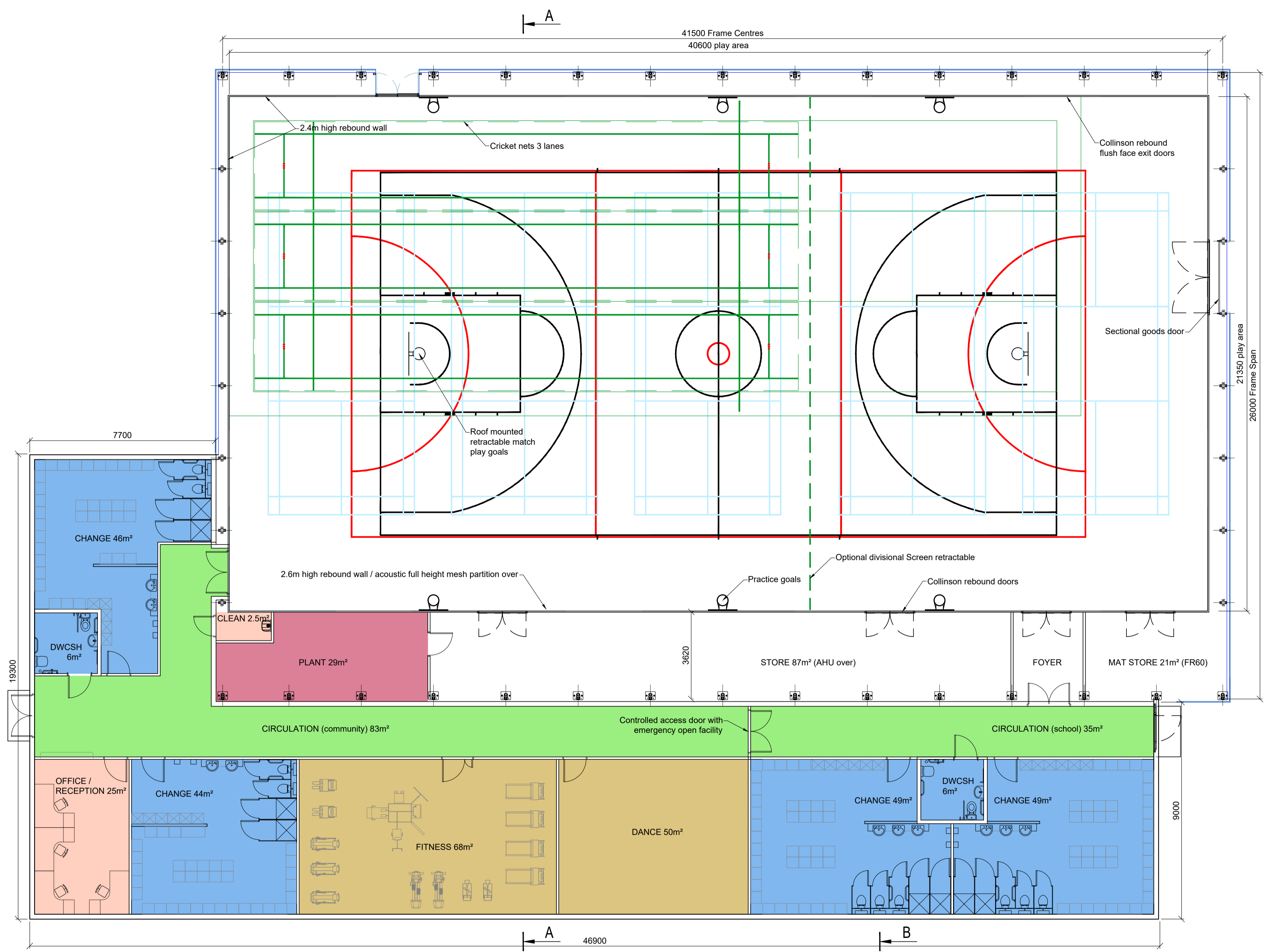
LAYOUT PLAN
